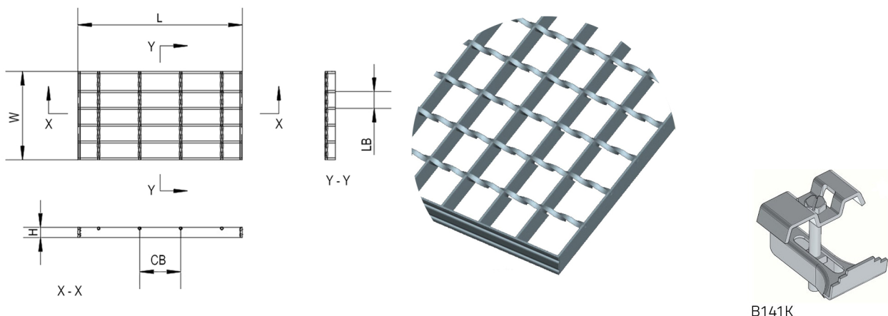
Fixing Types
